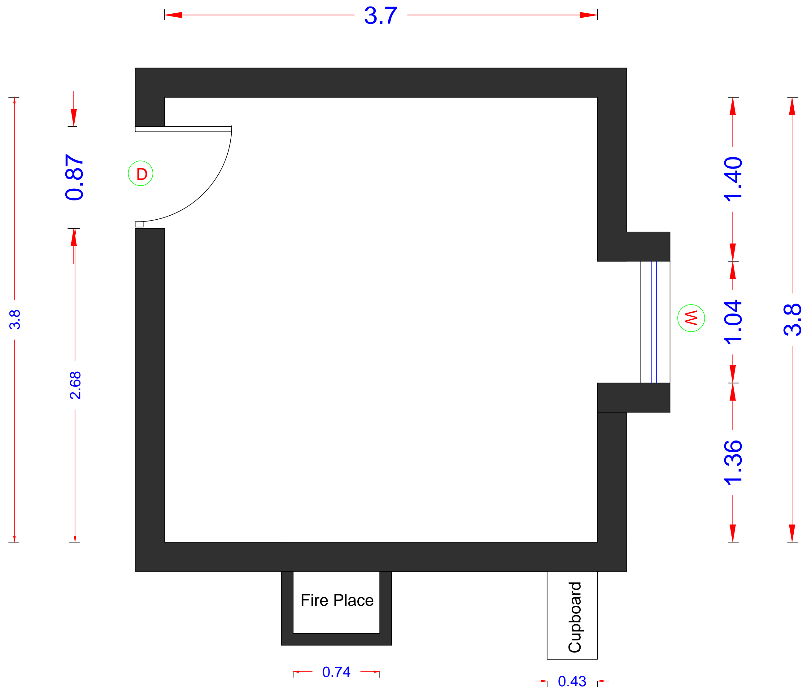
FLOOR PLAN
