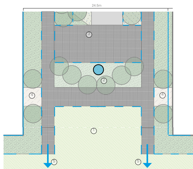
Plan; node where residential street meets linear park
