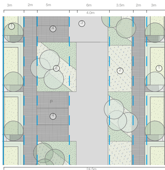
Typical street plan & cross section
